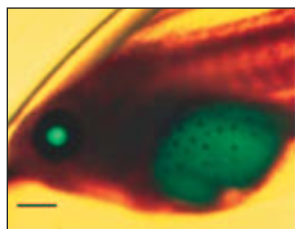
Transgenic (left) tadpoles express fluorescently tagged rhodopsin (green) in their eye, control (right).
